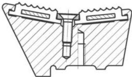
Replacement for existing pre-opening segment bars
