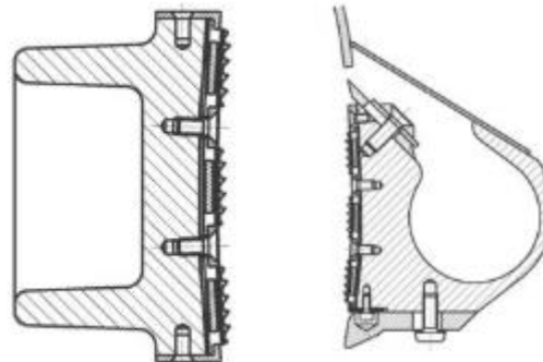
Conversion of existing carding plates to 3 stationary flats
