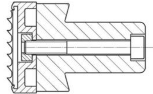
Conversion from clipped to screw-type fastening
